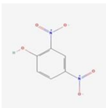
Figure 1: (A) Structure of the 2,4-Dinitrophenol (DNP) compound. (PUBCHEM, 2022).
